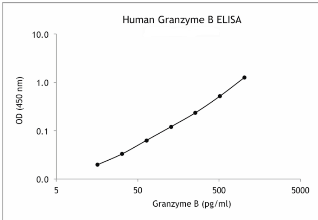
Example of a representative Human Granzyme B standard curve using a 4-parameter logistic fit.
