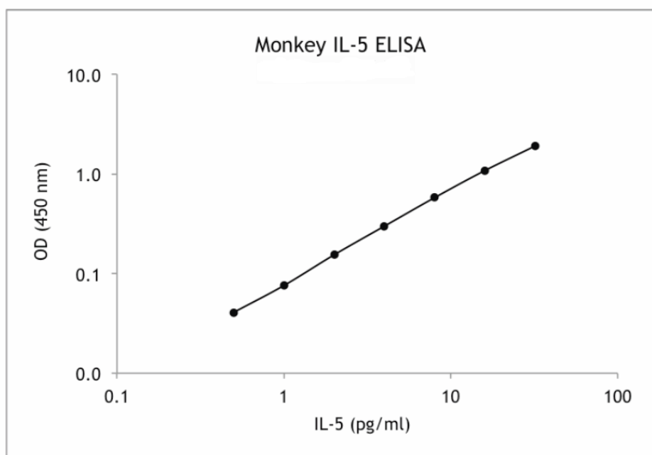
Example of a representative Monkey IL-5 standard curve using a 4-parameter logistic fit.
