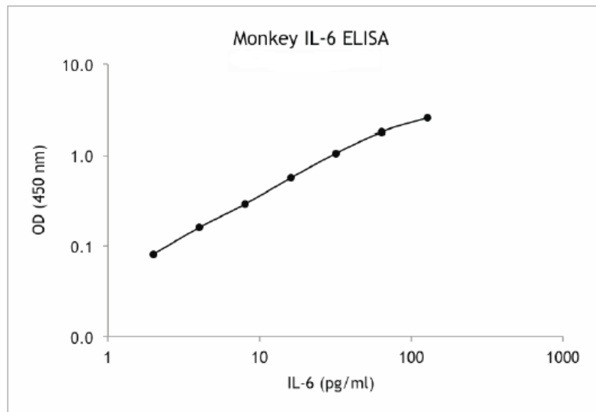
Example of a representative Monkey IL-6 standard curve using a 4-parameter logistic fit.
