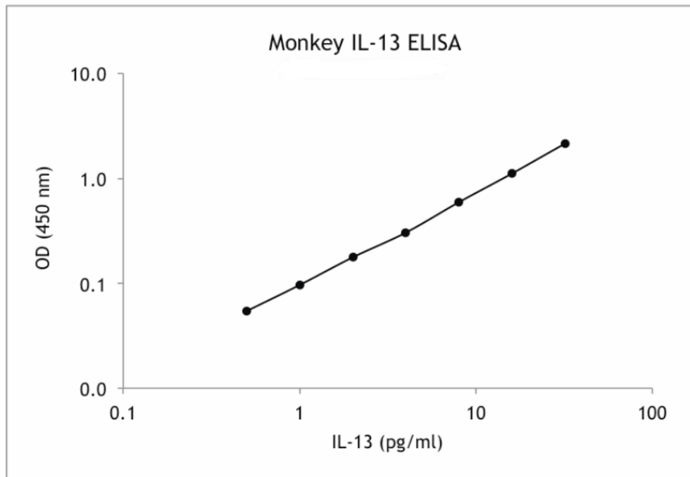
Example of a representative Monkey IL-13 standard curve using a 4-parameter logistic fit.
